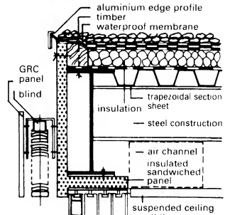
16 Indoor swimming pool with insulated sandwiched panel fascia
